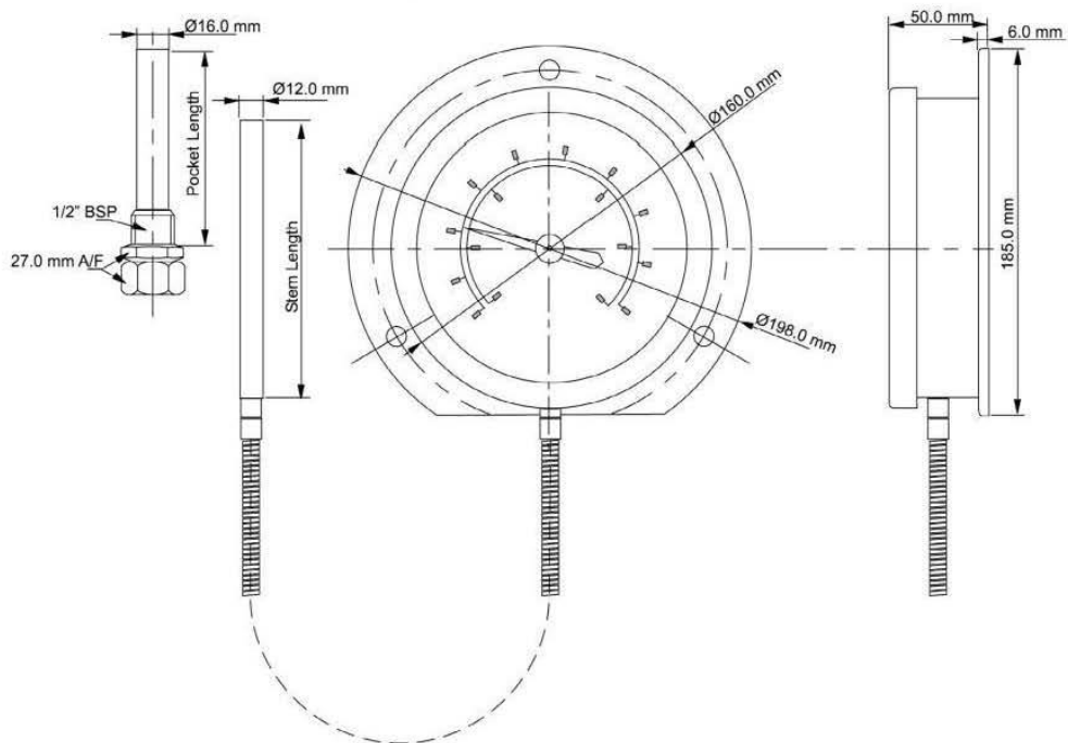
150mm Dial Thermometer - Bottom Entry
