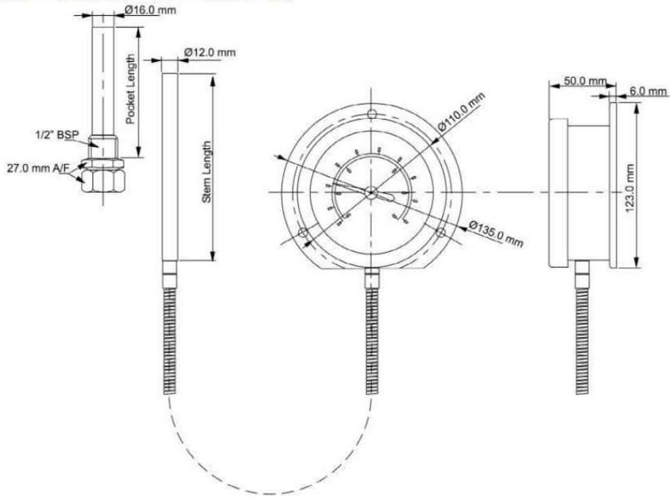
100mm Dial Thermometer - Bottom Entry
